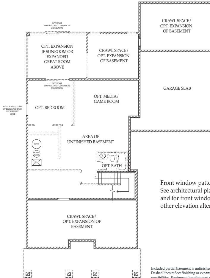
LOWER LEVEL FLOOR PLAN Opt. Media / Game Room or Sun / Screen Porch
