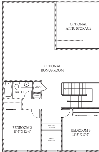
UPPER LEVEL FLOOR PLAN Upper Level Bonus Room Option
