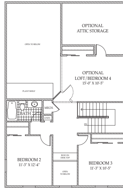
UPPER LEVEL FLOOR PLAN Opt. Loft / Bedroom 4
